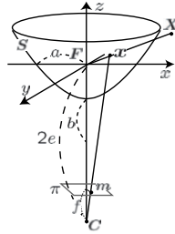
Figure 4: A hyperbolic-camera model. A point \mathbf{X} in a space is transformed to the point \mathbf{x} on the hyperboloid and \mathbf{x} is transformed to the point \mathbf{m} on image plane. The geometrical property of reflected ray constructs the camera model with a hyperbolic mirror.
