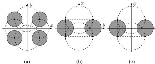
Figure 10: The gray circles in figures are the spheres. The dashed lines in these figures are the circles on a plane in a space. These spheres and circles are yielded by the collections of common points of three orthogonal planes selected from 28 epipolar planes.
