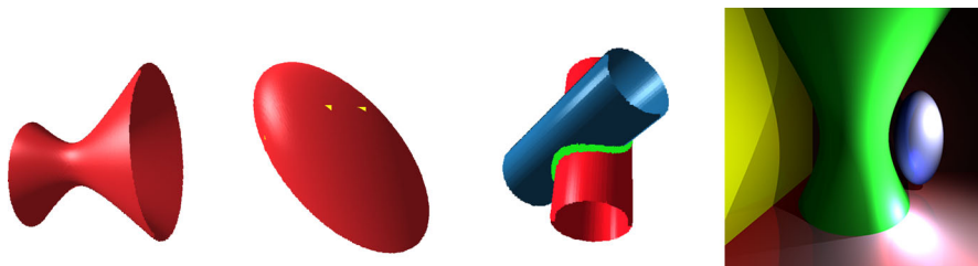
FIGURE 1. Example of our construction of QCGA objects. From left to right: a dual hyperboloid built from its equation, an ellipsoid built from its control points (in yellow), the intersection between two cylinders, and a hyperboloid with an ellipsoid and planes (the last one was computed with our ray-tracer)
